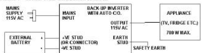
FIGURE 1 - CONCEPT AND CONNECTION DIAGRAM.
